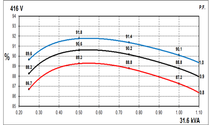
60Hz Curves
