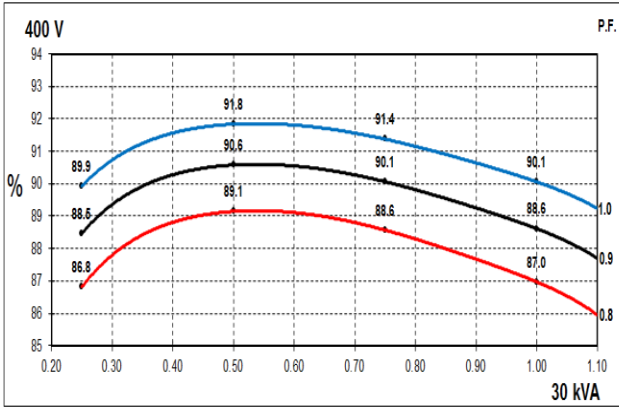
50Hz Curves
